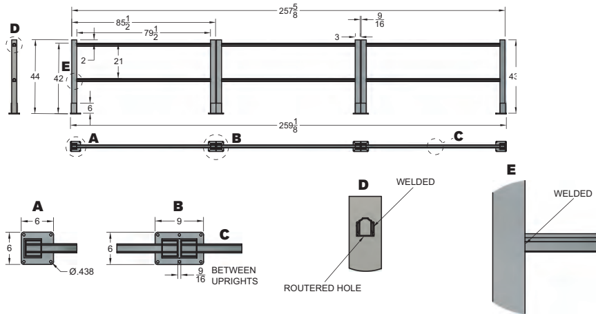
Stanchion Mounts
