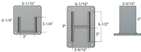
Stanchion Mounts
