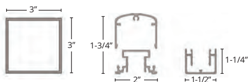
Routed Post
