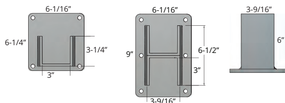
Stanchion Mounts
