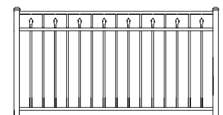
EFR-25
