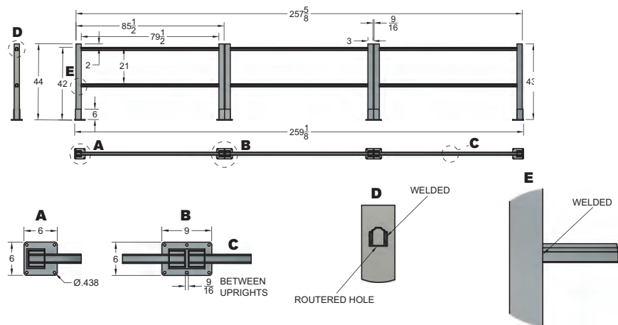
Stanchion Mounts
